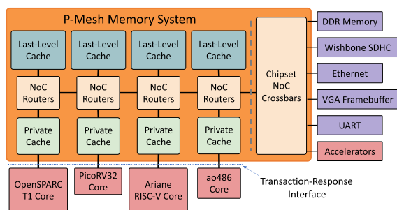
Figure 2. OpenPiton architecture, adapted. 1
