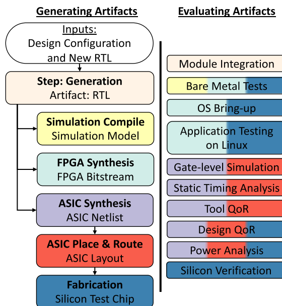
Figure 3. Artifact generation and evaluation using OpenPiton. Coloring of evaluation (right) corresponds with artifacts that may be used (left).
